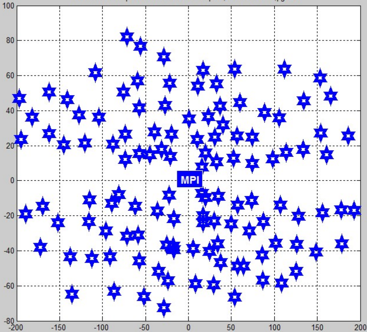
Locations of Impact to Mean Point of Impact; Data FM 6-40;pg 3-20
