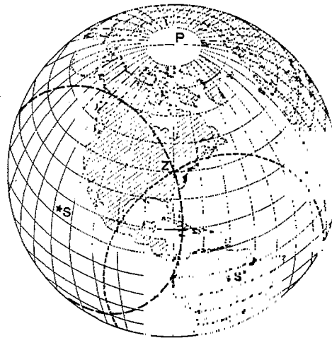
FIG. 2.—Circles of equal altitude
