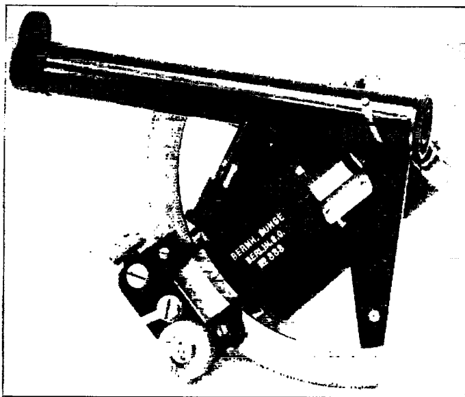
FIG. 6.—Lindt sextant
