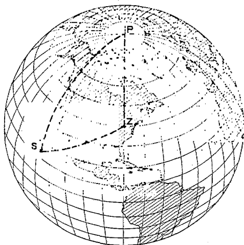
FIG. 1.—The astronomical triangle
