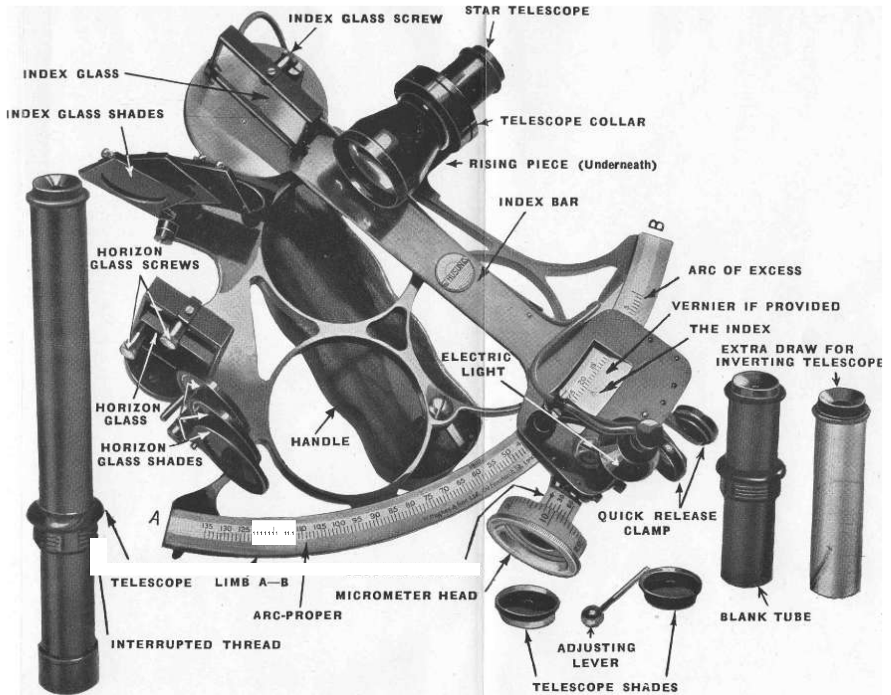
Fig. 3. A "3 Circle" Micrometer Sextant with the parts named.
