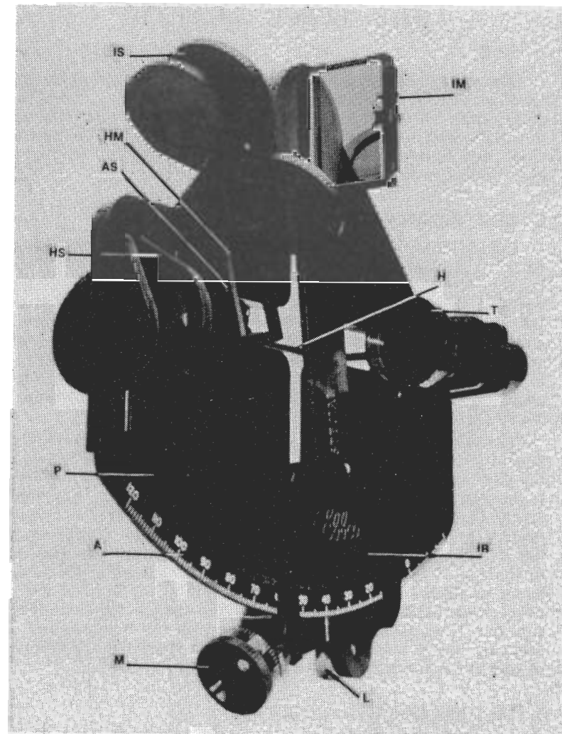
A: Arc I.B.: Index Bar P: Plate of Sextant H.M.: Horizon Mirror L: Lever T: Telescope I.M.: Index Mirror H.S.: Horizon Shades H: Handles A.S.: Adjusting Screws I.S.: Index Shades M: Micrometer Drum
