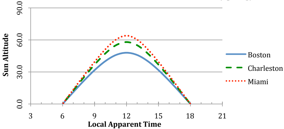
Sun Altitude vs Time for Different Locations (Spring)
