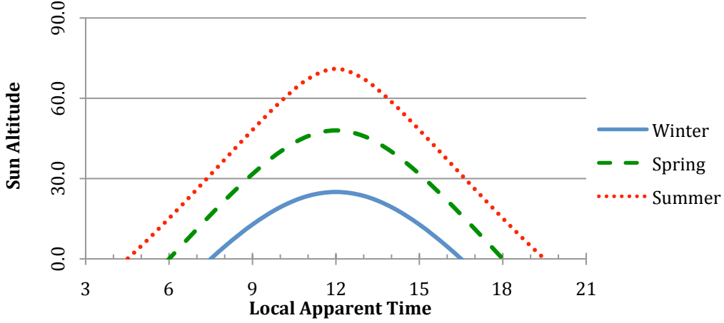
Sun Altitude vs Time for Different Seasons (Boston)
