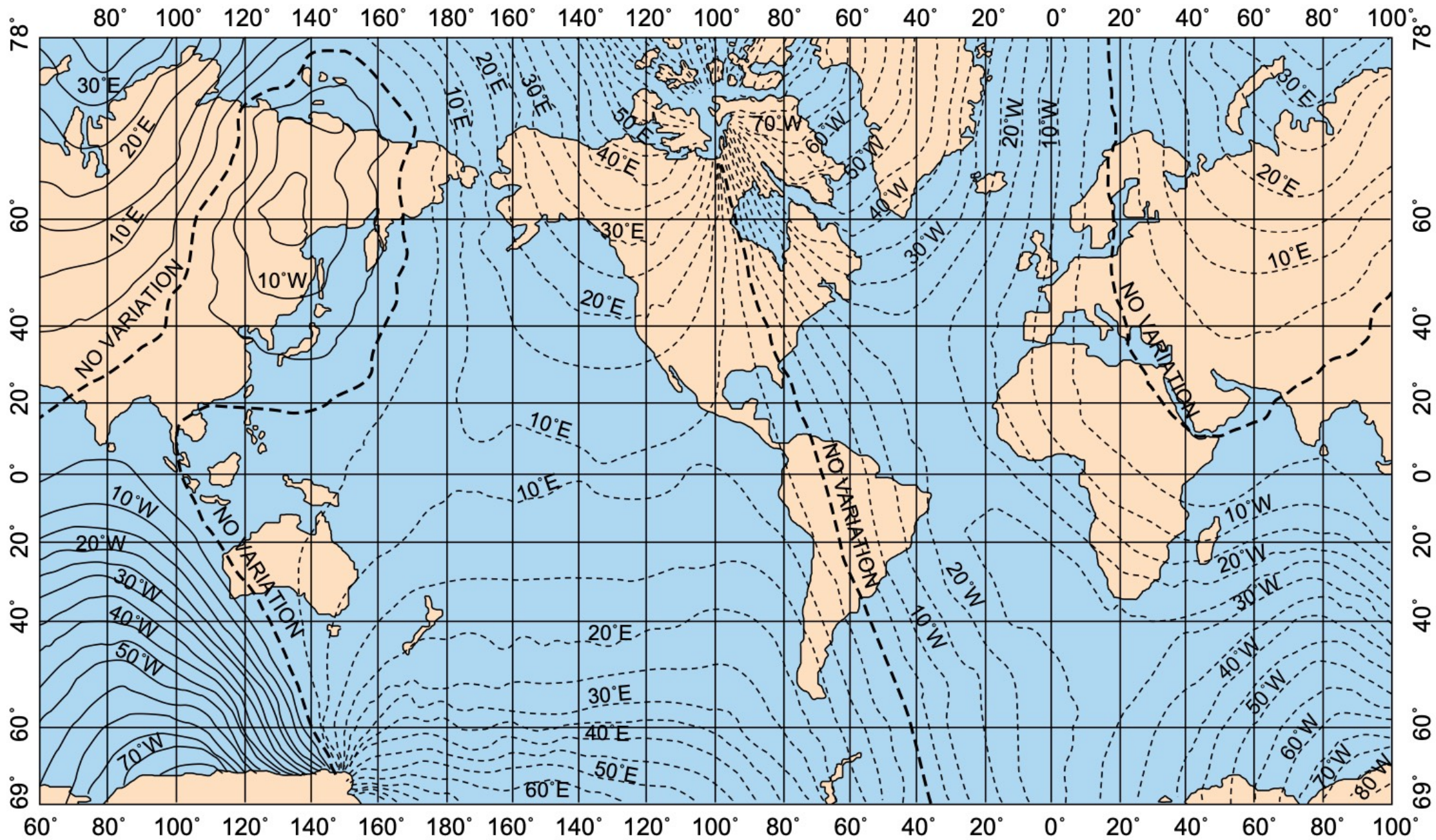
Figure 3-4. Isogonic lines show same magnetic variation.
