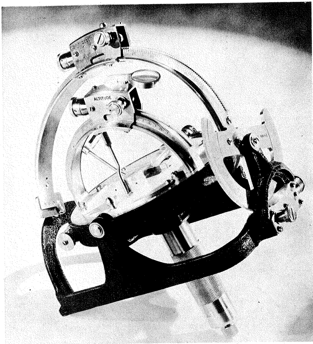
FIGURE 52.—Computing instrument.
