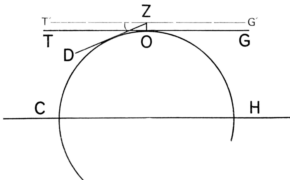
O:—Observer; C, H:—Celestial Horizon; T, G:—Tangent T', G':—Parallel to Tangent at H.E. Z:—Height of Eye; T', Z, D:—Angle of Dip
