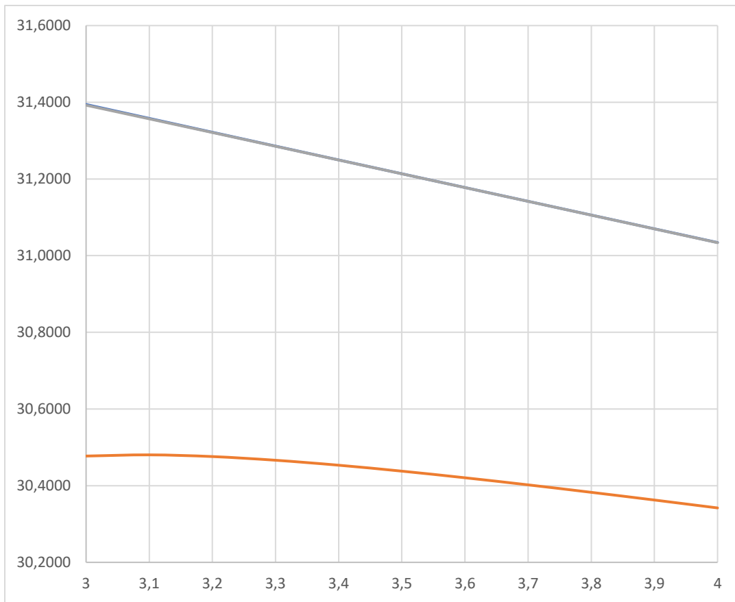
22 August 2022. Latitude 47°10'N, longitude 9°32'E. The upper curve shows the true (geocentric) distance between Moon's centre and Procyon, in degrees. The lower curve shows the apparent distance. The x-axis is hours UT.
