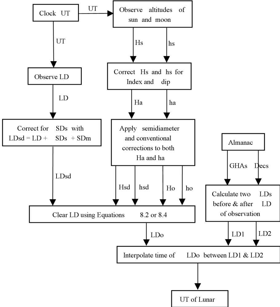
Figure 8.4. Flow chart for reducing a lunar distance sight.
