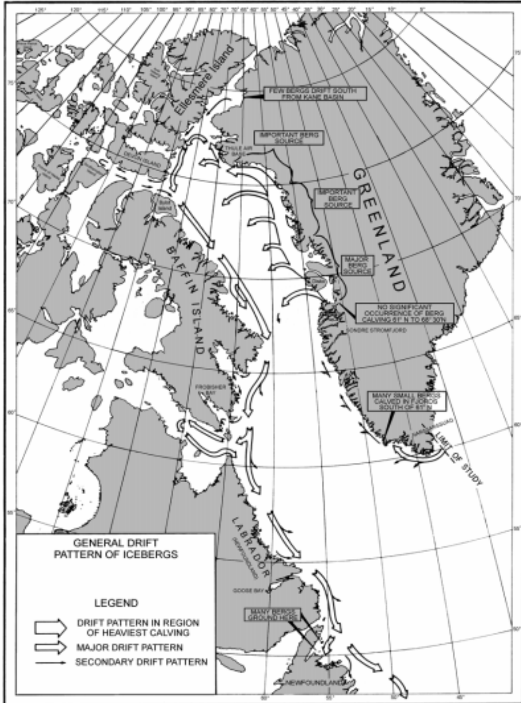
Figure 3410a. General drift pattern of icebergs.
