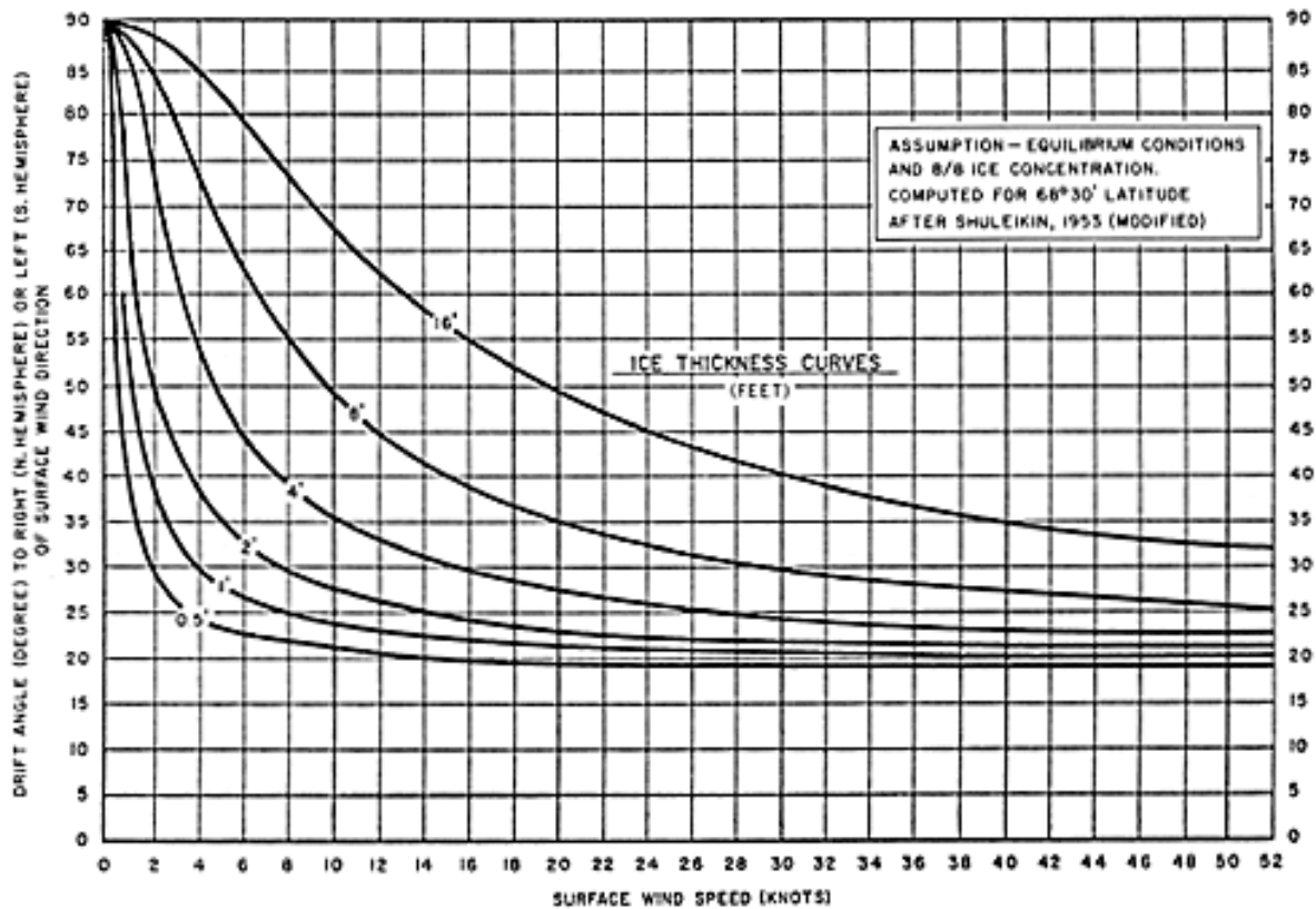
Figure 3407. Ice drift direction for varying wind speed and ice thickness.
