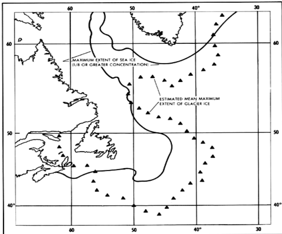
Figure 3410b. Average iceberg and pack ice limits during the month of May.
